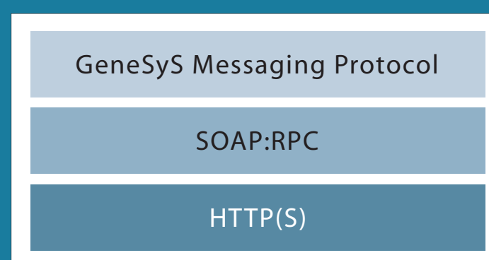
Messaging API
