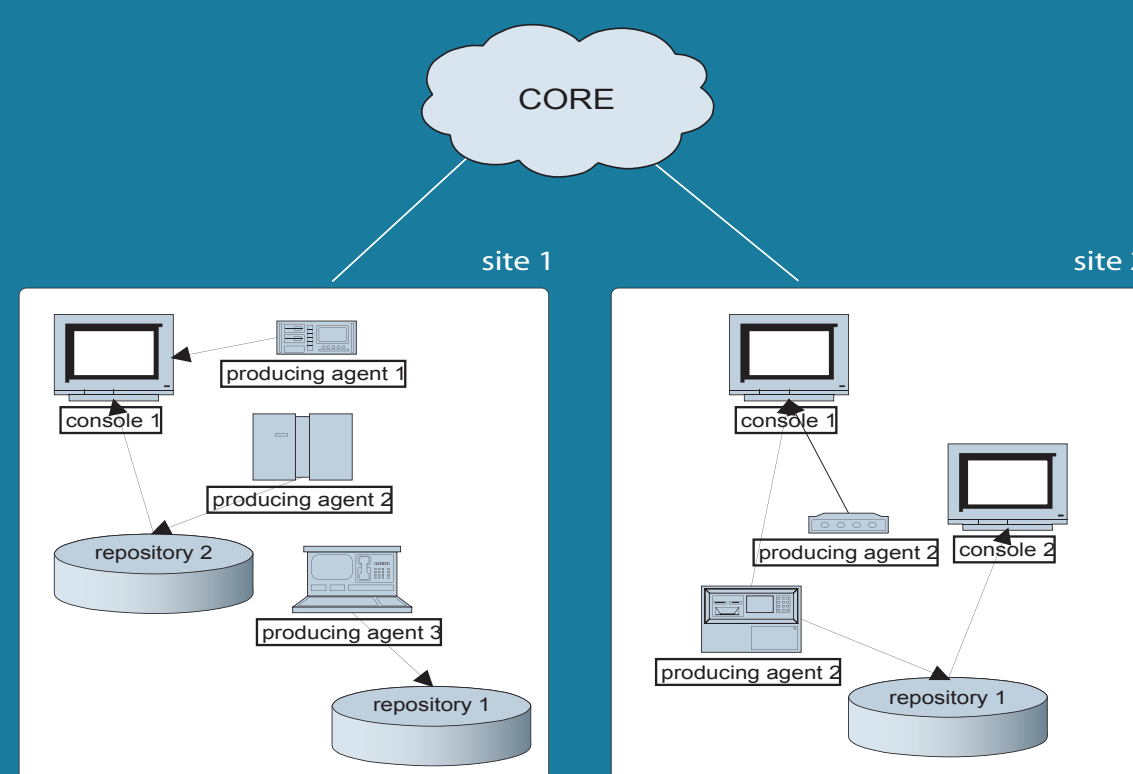
Component Model
